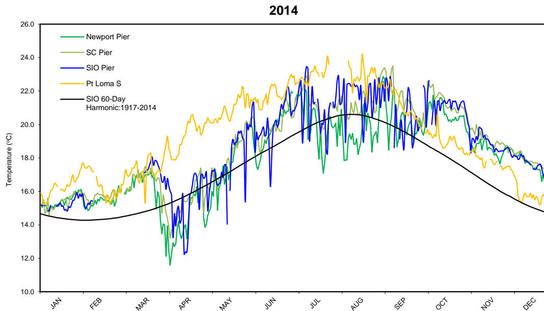
Figure 8. Sea surface temperatures (SST) at Newport Pier, San Clemente (SC) Pier, Scripps (SIO) Pier, and Point (Pt) Loma South (S) for 2014 compared to long-term harmonic mean from SIO Pier.
