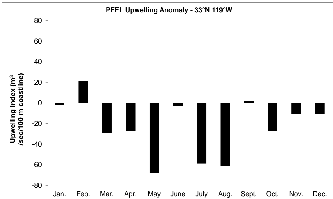
Figure 9. A) Daily Upwelling Index (UI) at 33°N 119°W. The dashed curve is a smoothed biharmonic fit to the daily UI from 1967–1991. The purple area represents one standard error, and the yellow bars are monthly means. Units are cubic meters per second per 100 meters of coastline. B) UI anomaly (2014 compared to the monthly mean from 1946–2013). Source: (NOAA PFEG 2015).
