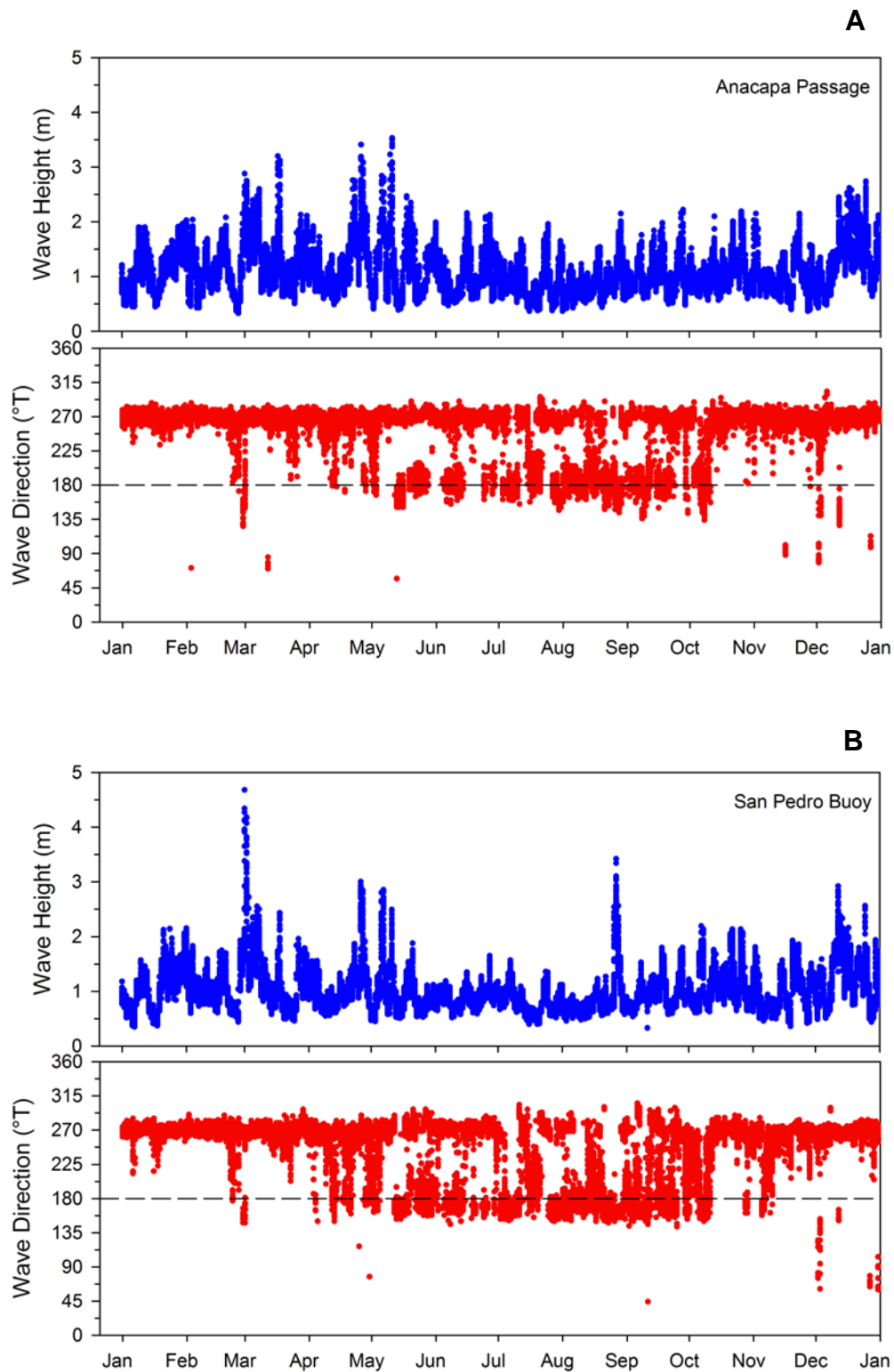
Figure 11. Wave height (blue) and direction (red) at A) Anacapa Passage Buoy and B) San Pedro Buoy from January 2014 through December 2014. Data from CDIP (2015).
